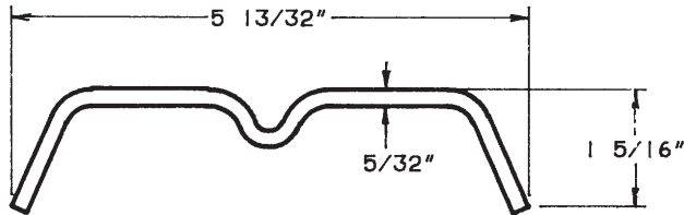
T-4 4 Lbs. Per Foot
