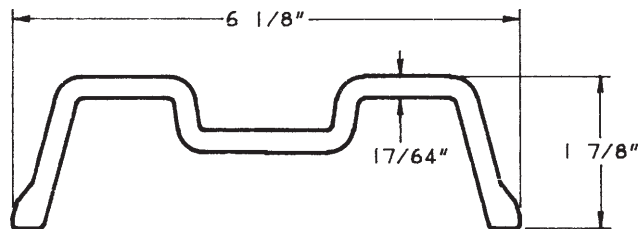
T-9 9 Lbs. Per Foot
