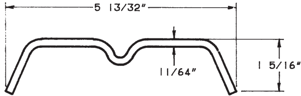
T-5 5 Lbs. Per Foot
