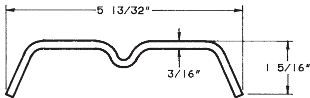
T-6 6 Lbs. Per Foot
